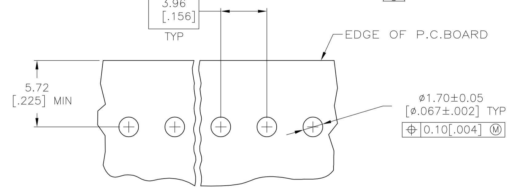
RECOMMENDED MOUNTING HOLE PATTERN FOR 1.57 [.062] THICK P.C. BOARD 10
